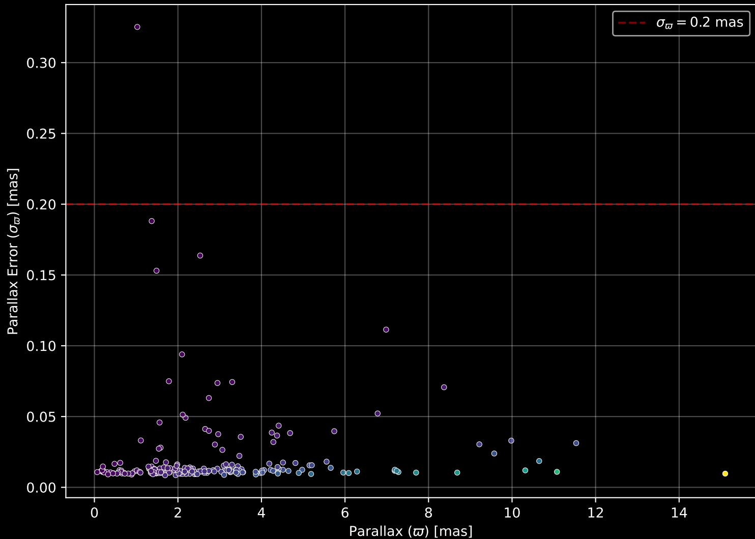
APOGEE DR17 Field: [273-41-O_TESS] Parallax Quality (n= 206)
