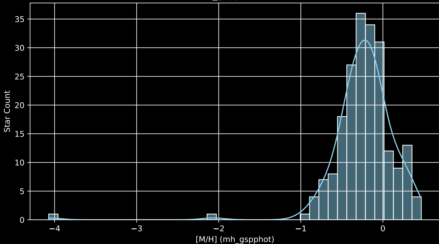
APOGEE DR17 Field: [273-41-O_TESS] [M/H] (mh_gspphot) (n= 206)
