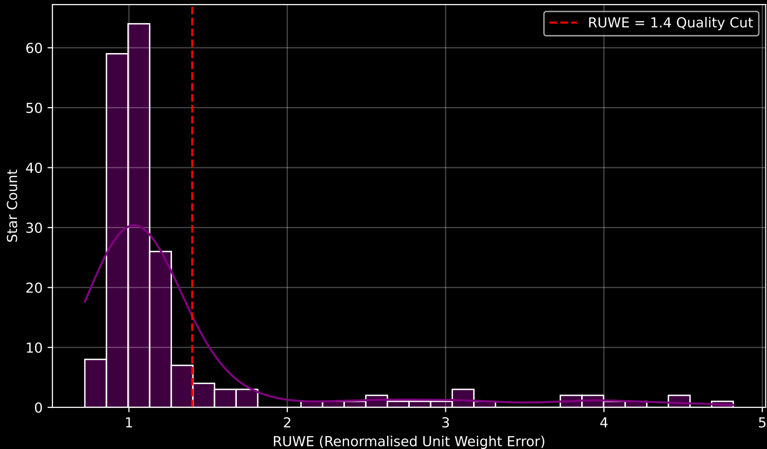
GAPOGEE DR17 Field [273-41-O_TESS] RUWE Distribution (n= 195)
