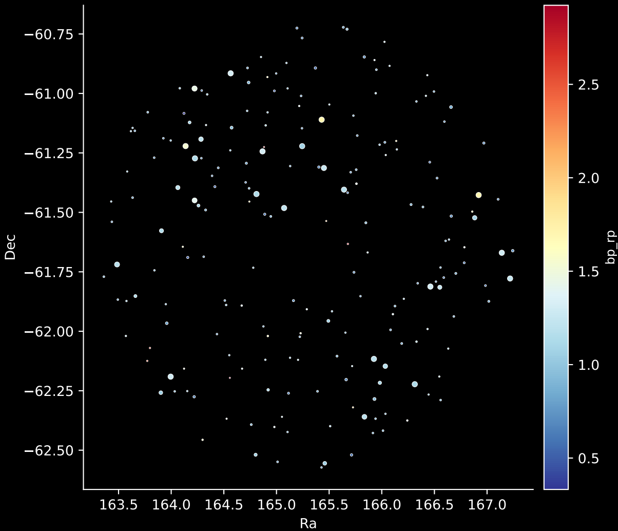
APOGEE DR17 Field: [273-41-O_TESS] Stars: 206
