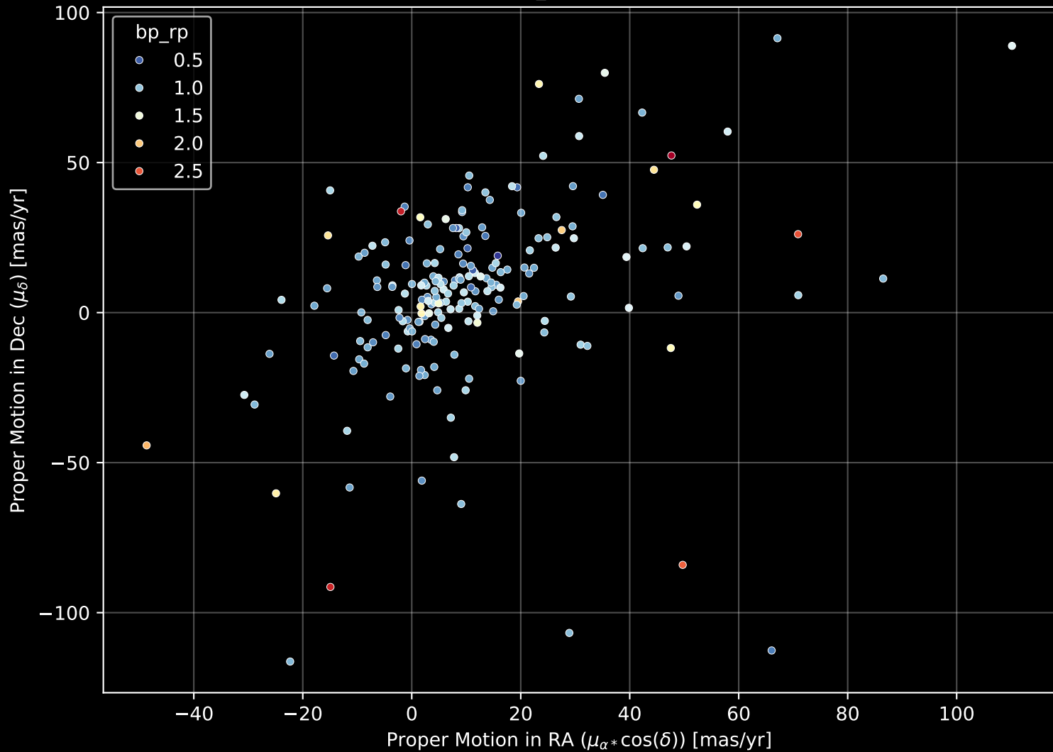
APOGEE DR17 Field: [273-41-O_TESS] Proper Motion Diagram (n= 206)
