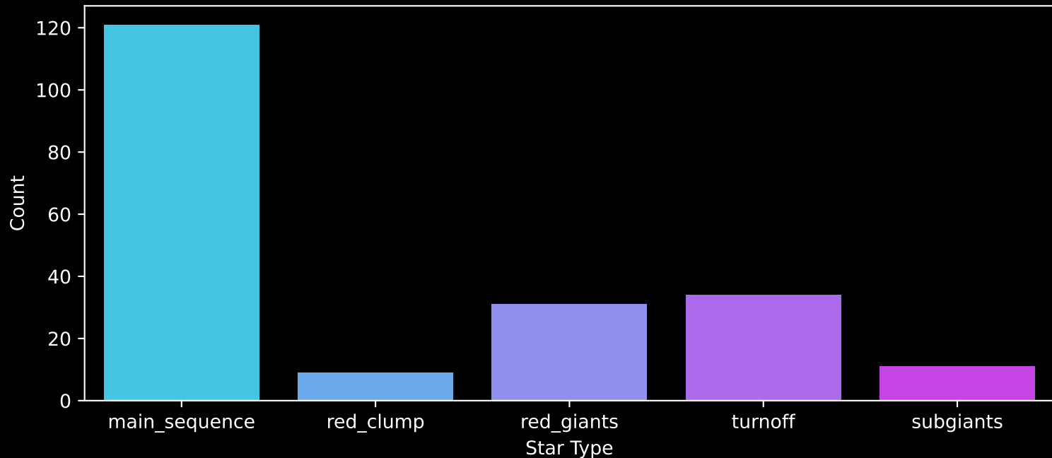
APOGEE DR17 Field: [273-41-O_TESS] Count plot of Star Type
